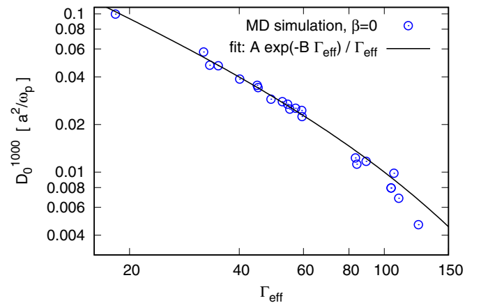
FIG. 5. Fixed-time ( t\omega_p = 1000 ) diffusion coefficient, D_0^{1000} , from the \beta = 0 reference simulations as a function of the effective Coulomb coupling parameter. The theoretical fit formula is adapted from Ref. [46] with A = 2.1444 and B = 0.00778 .
