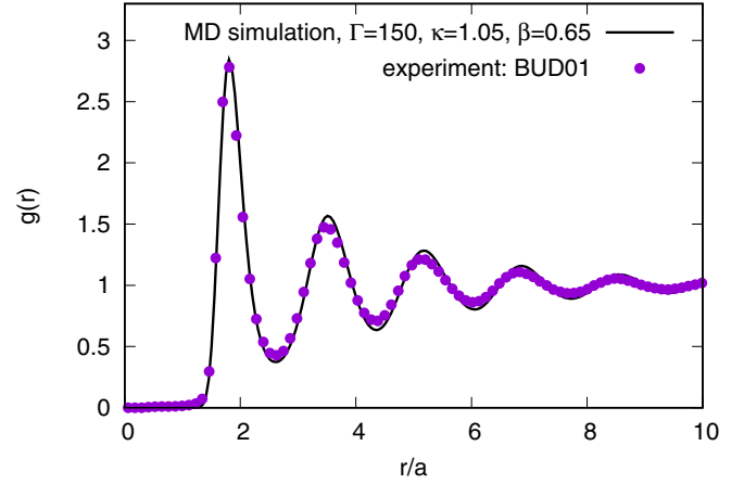
FIG. 3. Pair correlation functions g(r) from the experiment (BUD01, symbols) and MD simulation (line) with parameters \Gamma = 150 , \kappa = 1.05 , \beta = 0.65 .
